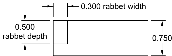
RABBET DETAIL
